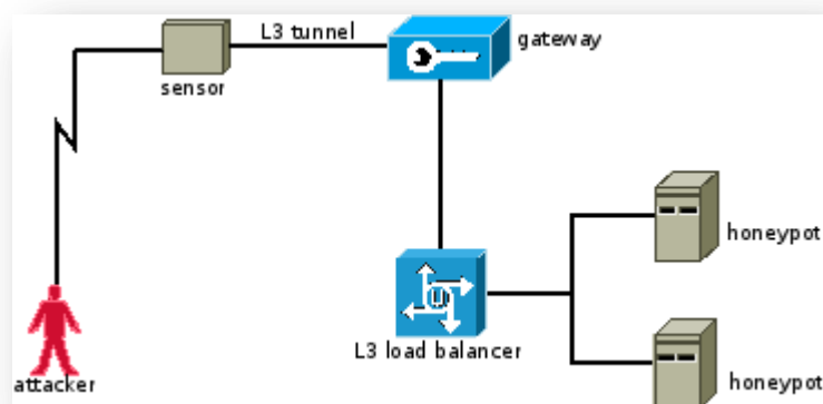
Figure 6: A thin sensor architecture
