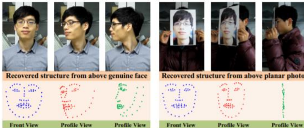
Figure 22: A comparison of recovered sparse 3D facial structures between genuine and photo face, showing significant differences 25
