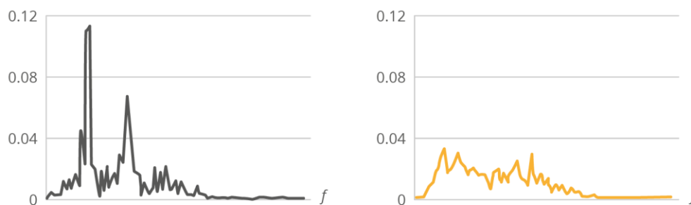
Figure 21: Typical power spectrum distribution patterns of a real access (left) and a mask attack (right) extracted from the green colour channel 24
